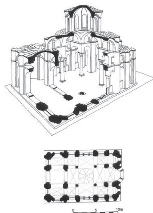
FIG. 1. Cutaway perspective view of the Myrelaion (Baburn Camii), Istanbul FIG. 2. Plan of the Myrelaion
